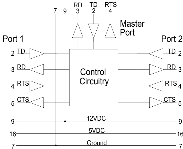
232PTC Port Diagram
