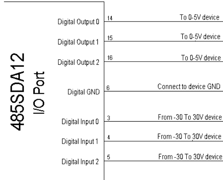
Figure 2.2 - Typical Digital I/O Connections
